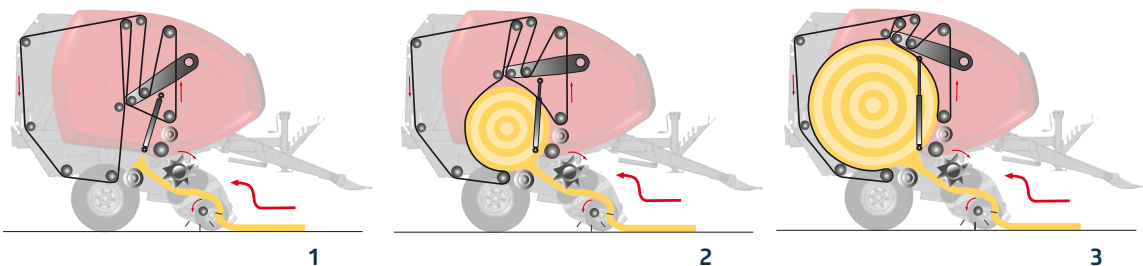
A combination of 5 belts and three rollers provides dense bales with a soft core and an easy bale start.
